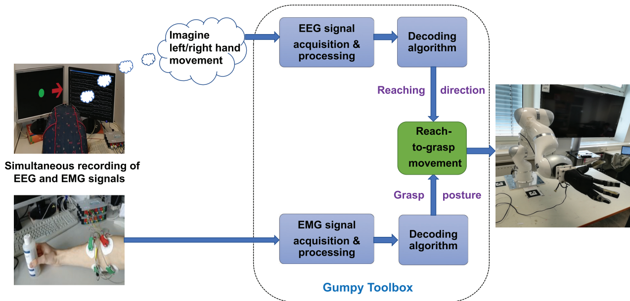
Figure 13. The proposed hybrid BCI experiment for reach-to-grasp movements decoding.
