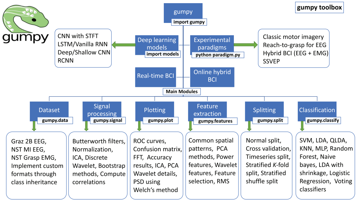
Figure 1. Overview of gumpy toolbox modules and functions.
